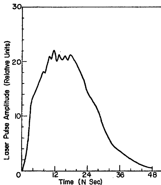
FIG. 1. Laser pulse history.
