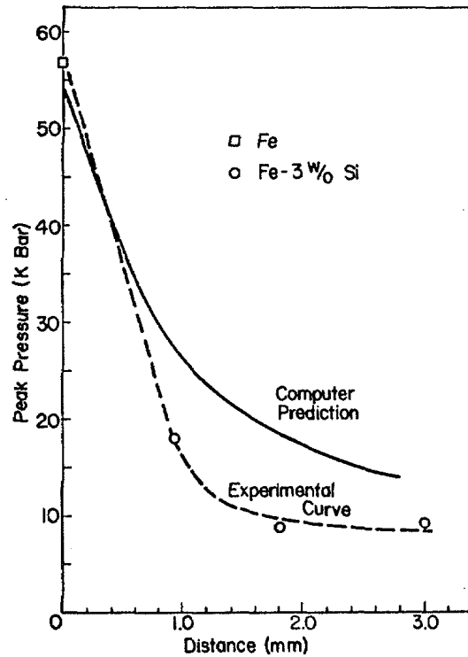
FIG. 2. Peak pressure attenuation in iron-3 wt% silicon.
